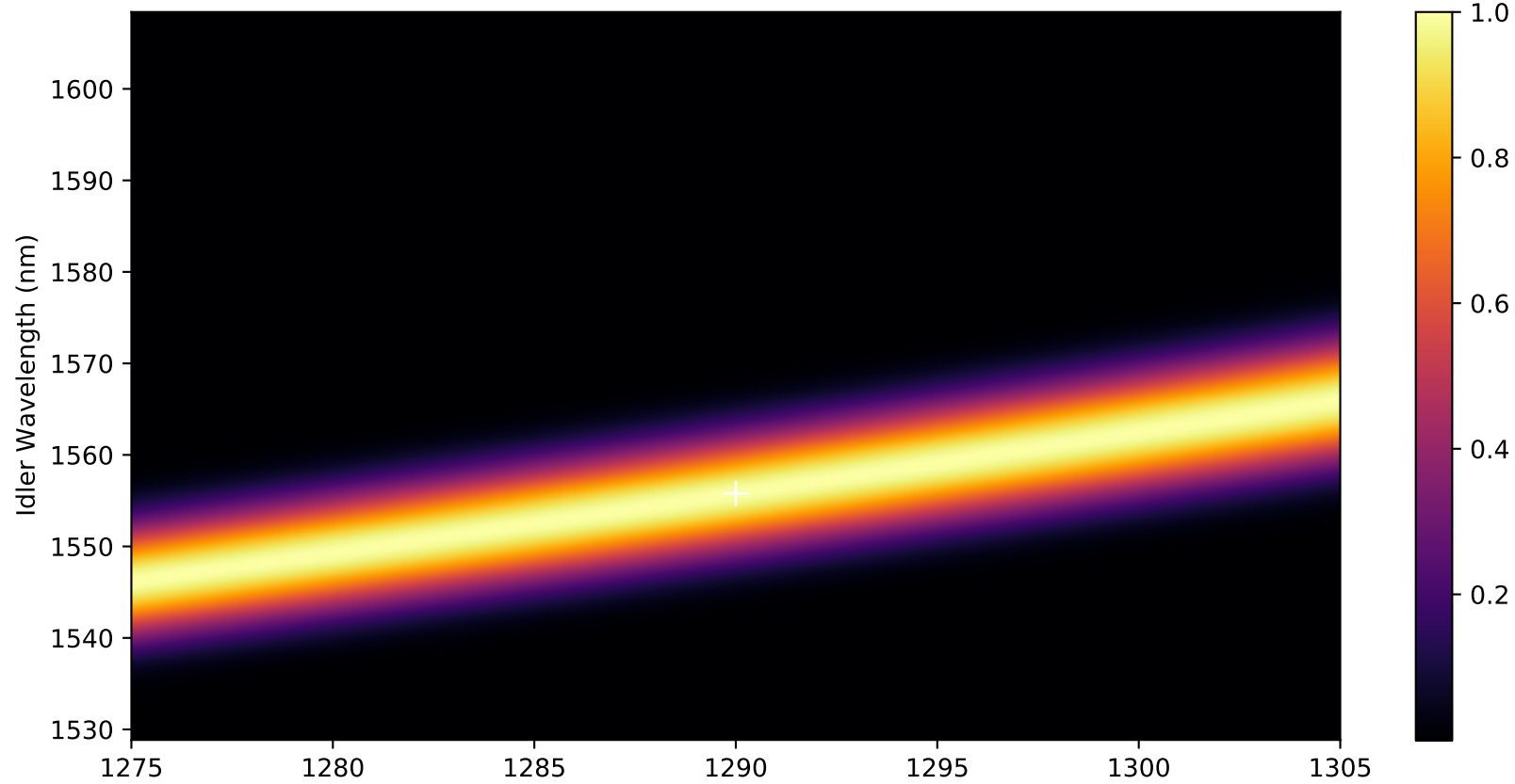
3. Optimized JSA (Theory) Pump=4.40nm | Purity=0.9978
