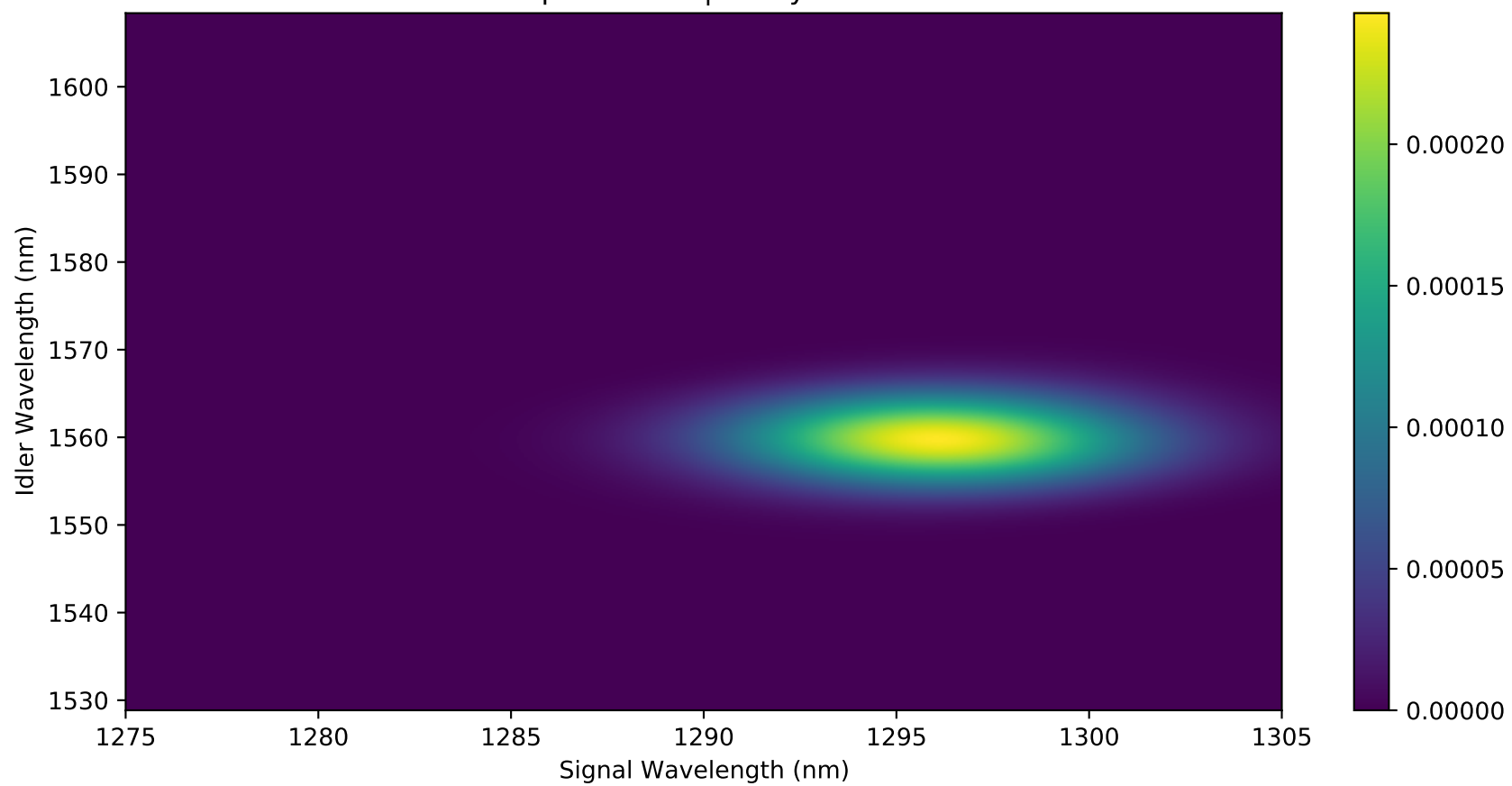
3. Optimized JSA (Theory) Pump=4.40nm | Purity=0.9978
