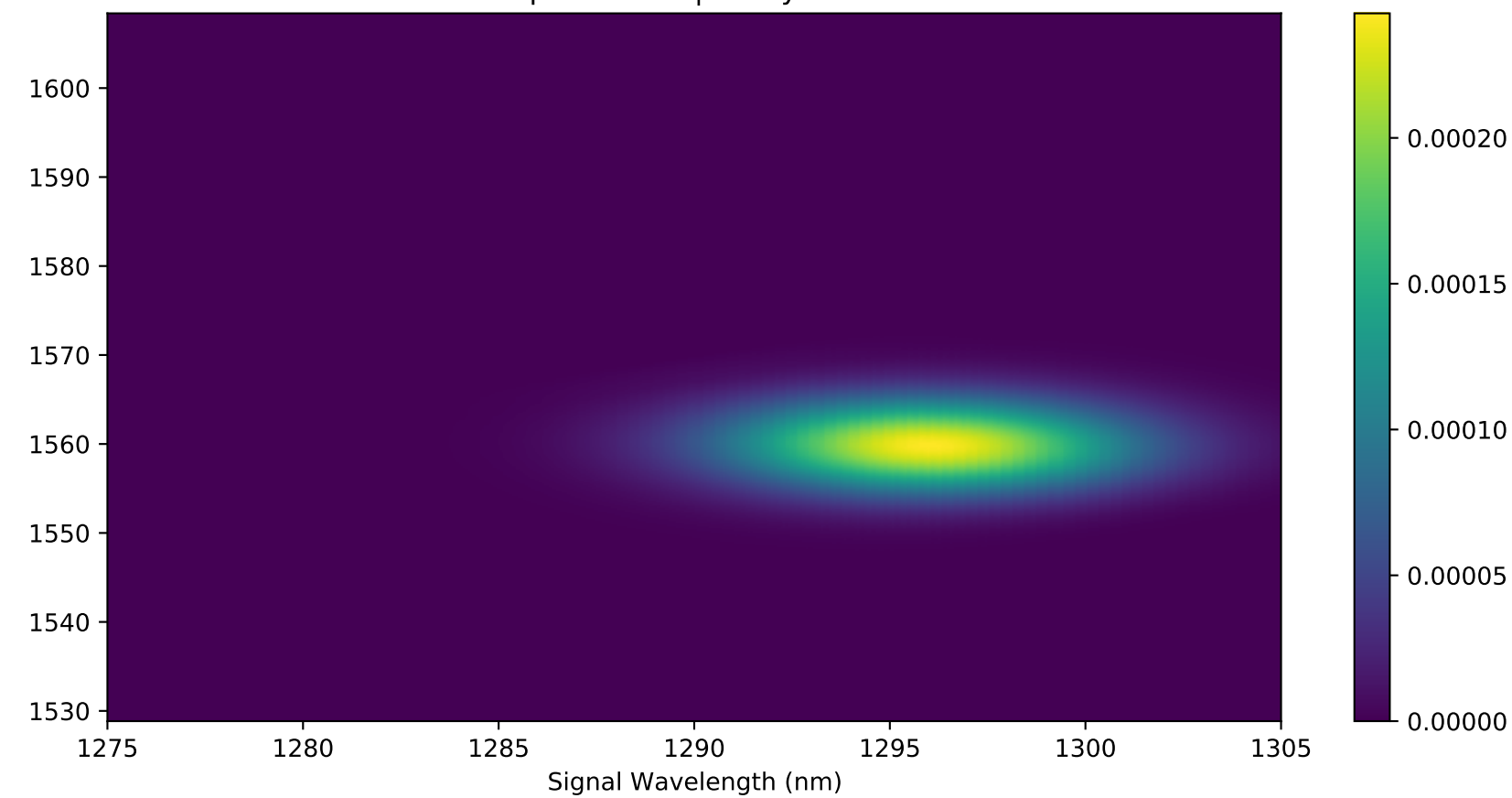
4. Optimized JSA (Exp Reconstruction) Pump=4.40nm | Purity=0.9967
